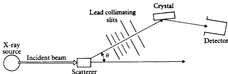
1.10 Schematic diagram of Compton's apparatus.
